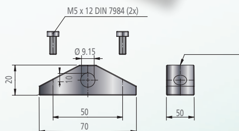
Wall mounting bracket item no. 503 895 For mounting in front of wall openings Material: Anodized aluminum
