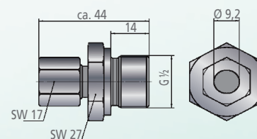
Through-bolt joint item no. 532 160 For gas-tight mounting in tubes and channels; atmospheric pressure Material: Stainless steel 1,4571, clamping ring PTFE
