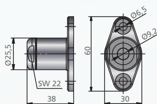
Wall mounting flange item no. 520 181 For mounting on walls through wall openings Material: Stainless steel 1,4571, PTFE
